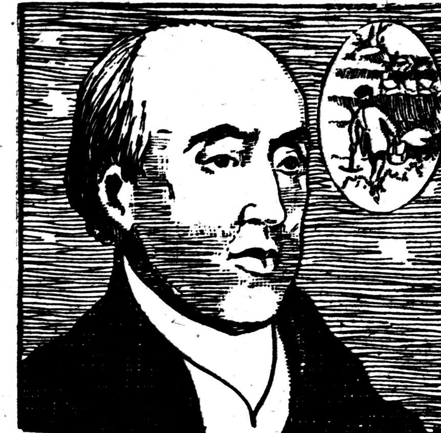
James Hutton, a doctor by profession, laid the cornerstone of modern geological thought when he declared that all changes in the earth's surface must be explained in terms of such forces as can now be observed at work. He was born in 1726 and died in 1797.
