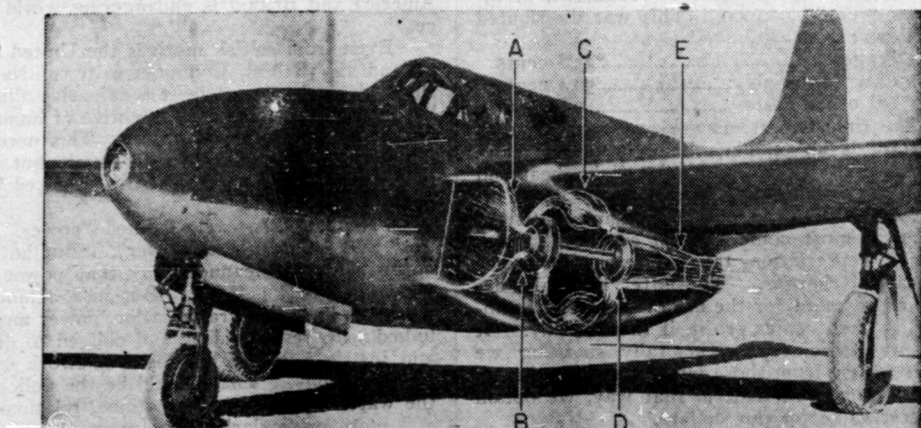
Simplicity of jet motors is indicated in this sketch of the P-59-A propellerless fighting plane. Note that basically the motor consists of a drive shaft, impeller and turbine wheel. Air flows into intake (A), is compressed by impeller (B), and goes to blast chamber (C), where fuel is ignited and temperature raised. Turbine (D) is propelled by air pressure and in turn gives power to air compressor at front of engine. Air flows at high velocity through nozzle (E) creating by reaction the force which drives plane forward. This plane uses twin turbo-jet engines.
