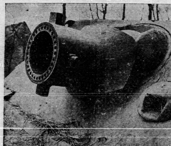
Looks more like something that mixes cement than what it is—a 380-mm. mortar mounted on a modified Mark VI German tank, captured by the Allies in Oberembt, Germany. The mortar barrel is seven feet long, and fires a five-foot shell weighing 770 pounds. Five-man tank crew protected by 5-inch armor in front.
