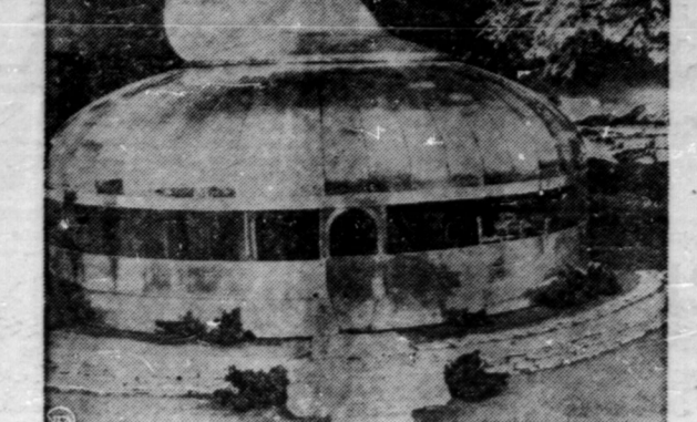
R. Buchmeister Fuller, Wichita, Kans., designed this hemispherical house from the inside out. Based on aircraft principles, the house weighs only 8000 pounds, packs into cylinder 16 x 4 1/2 feet.
