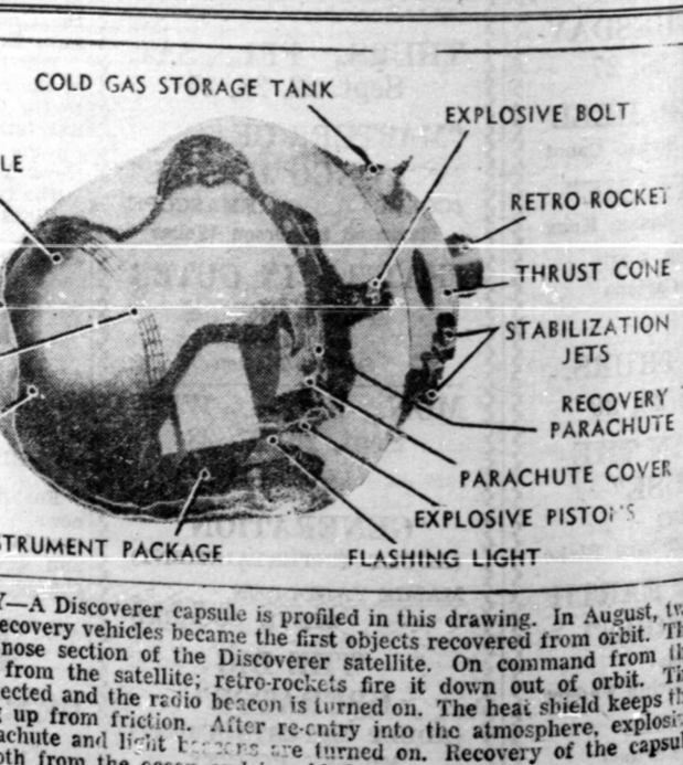
CAPSULE CUTAWAY — A Discoverer capsule is profiled in this drawing. In August, two similar re-entry and recovery vehicles became the first objects recovered from orbit...'
