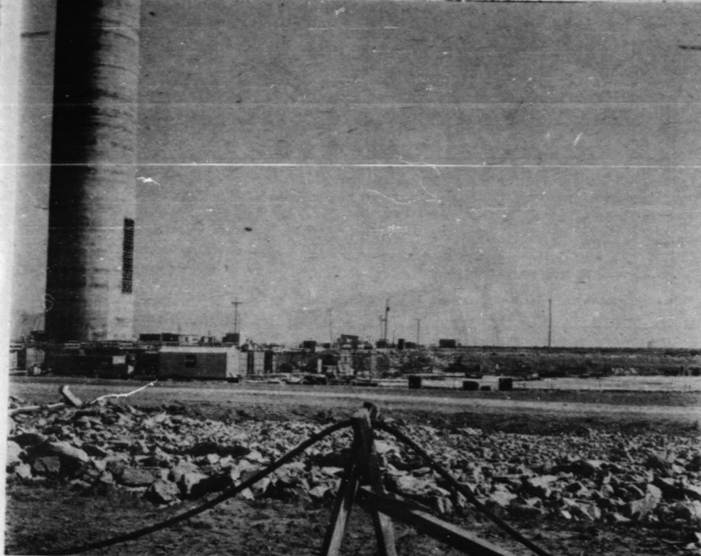
Not all of the 768 acres at Nanticoke's hydro site is being developed. On the east side of the 655-foot stack there is room to double the size of the 2,000,000 kilowatt plant. If the plant is extended to its maximum size it will be 910 feet long and 275 wide or three football fields long and one football field wide. The station will house four giant generators that will have capacity roughly equal to Canada's share of the power resources at Niagara Falls. (Staff Photo)
