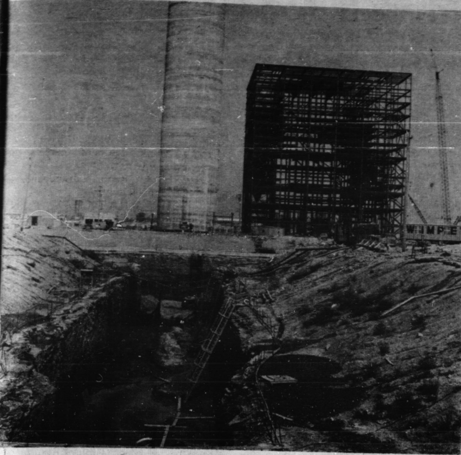
North from Lake Erie is this view of the Nanticoke Generating Station showing the main power plant and a portion of the 655-foot four-flue chimney. In the foreground is the intake canal which will draw 1,000,000 gallons of water per minute from the lake to serve the plant.
