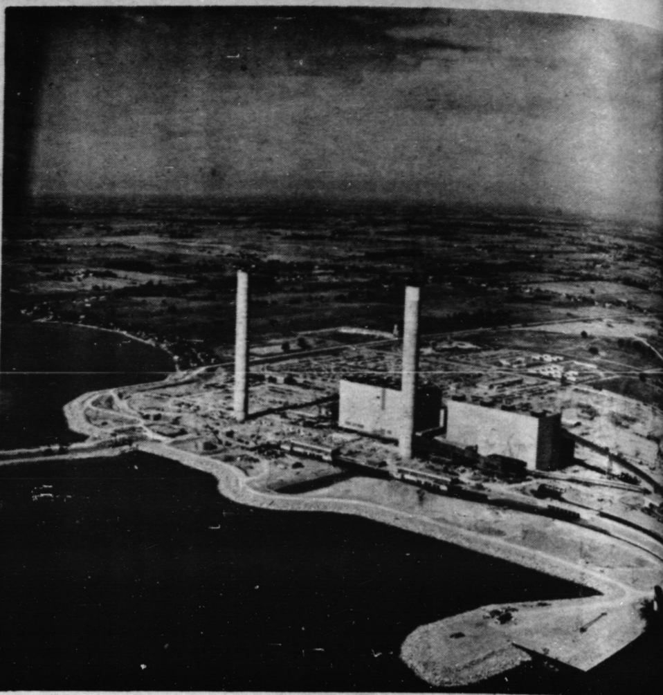
The two 650 foot stacks at Ontario Hydro's generating station at Nanticoke are completed, along with the first half of the building. The aerial photo shows how the new station looks as it gets ready to generate its first power later in December. (Ontario Hydro Photo)
